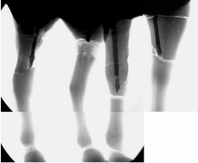
Fig. 10 Digitally composed X-radiograph of the horse (fig. 1, v).
